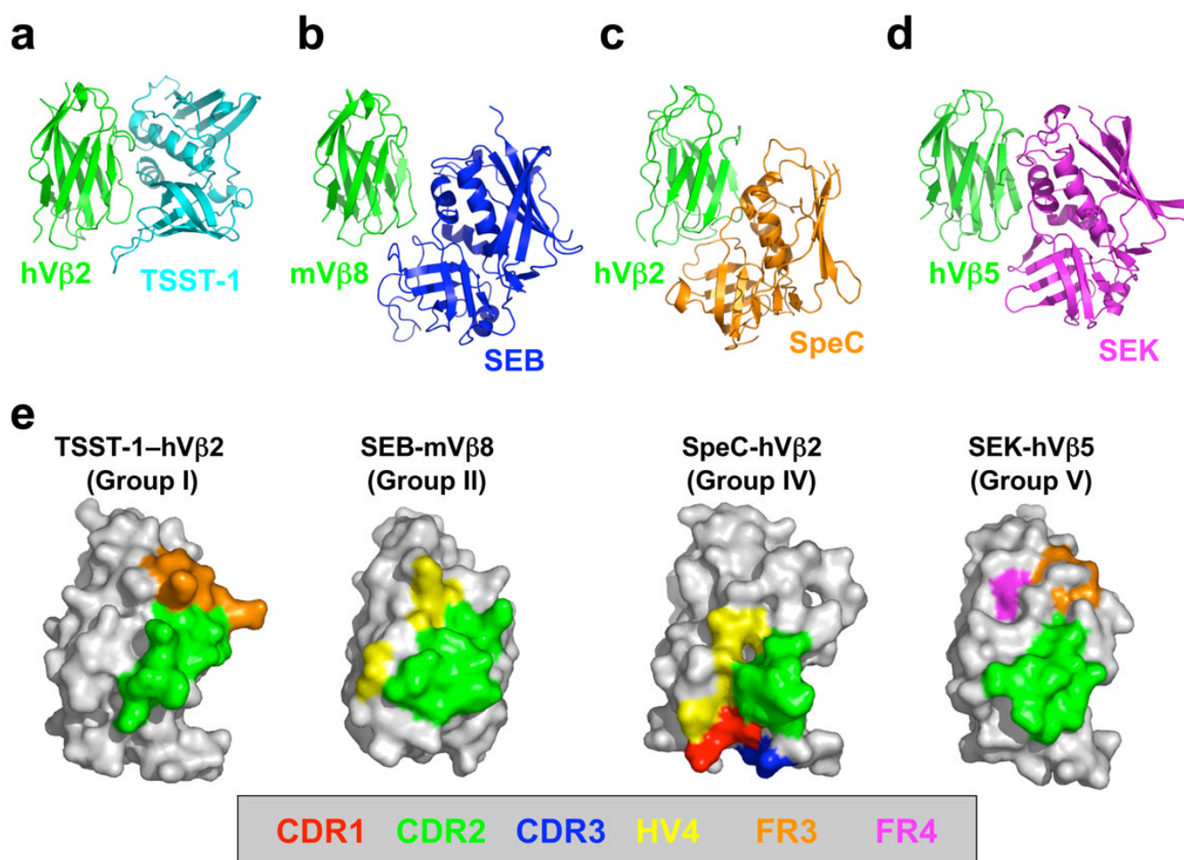
Fig. 3. Superantigen engagement of the T cell receptor V \beta domain. Structures of the (a) TSST-1/hV \beta 2, (b) SEB/mV \beta 8, (c) SpeC/hV \beta 2, and (d) SEK/hV \beta 5 complexes. The V \beta domains in panels a-d are aligned to one another to highlight the distinct orientations by which these SAGs engage their TCR ligands. (e) TCR V \beta domain molecular surface buried by various SAGs. Hypervariable and framework region surface residues buried in the interface formed by TSST-1, SEB, SpeC and SEK are color-coded as follows: CDR1 (red); CDR2 (green); CDR3 (blue); HV4 (yellow); FR3 (orange); and FR4 (magenta). The V \beta domains in panel e are rotated counter-clockwise approximately 90° about the vertical axis of the page relative to their positions in panels a-d.
